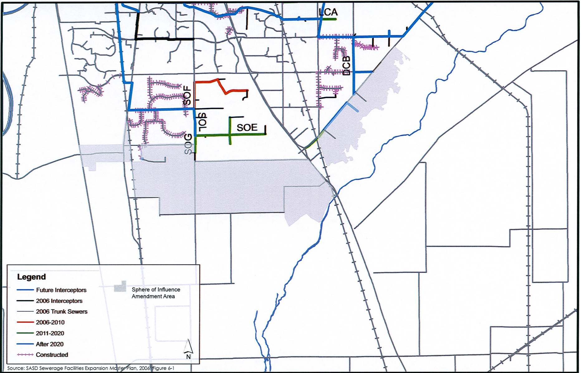
Figure 4.2-2 SASD Expansion Trunk Projects
